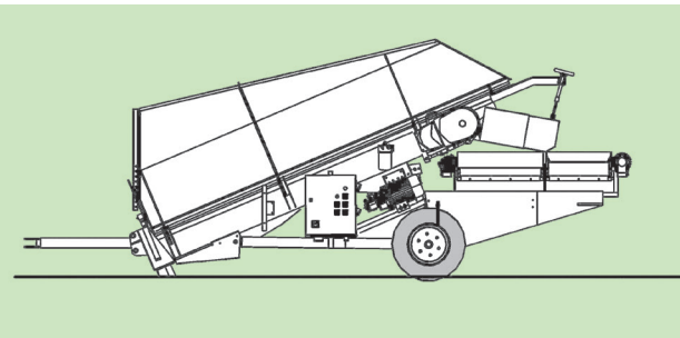
CSB 700/840-E
